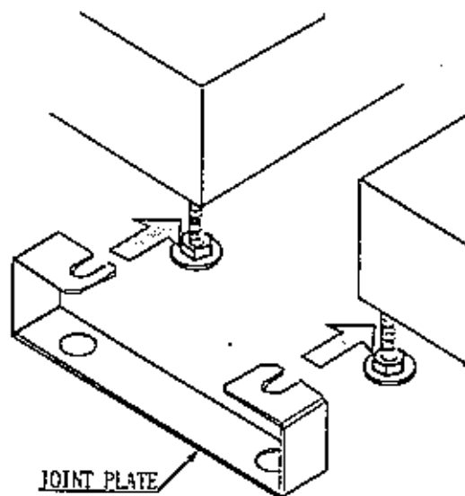
FIG. 6.6 LEG ADJUSTER
