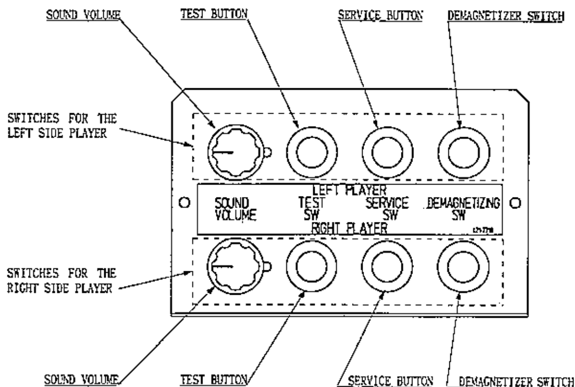
FIG. 8.1 SWITCH UNIT
